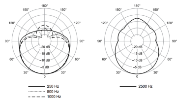
Polar Pattern
