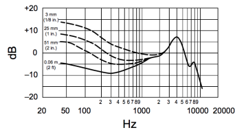
Frequency Response
