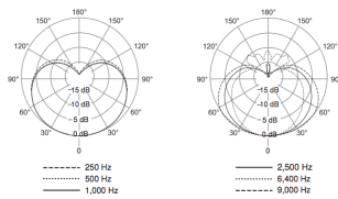
Polar Pattern
