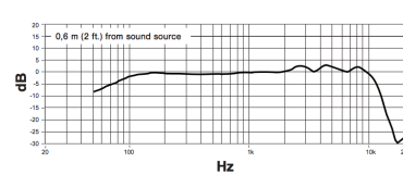
Frequency Response
